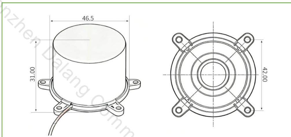
Figure 2 Product structure diagram (mm)
