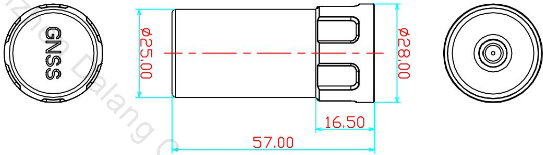
Figure 2 Product structure diagram
