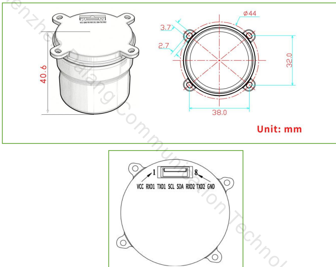
Figure 2 Dimensional Drawing (in millimeters)
