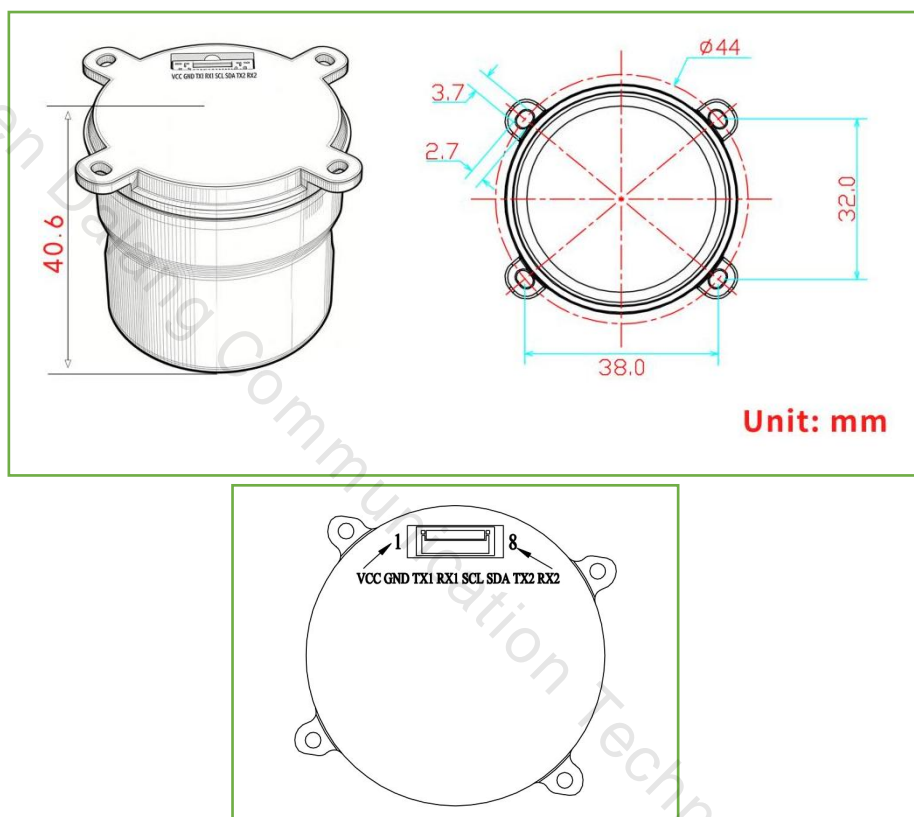
Figure 2 Dimensional Drawing (in millimeters)
