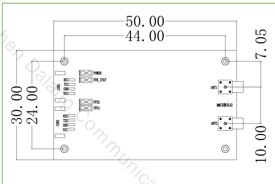
Figure 2 Dimensional Drawing (in millimeters)
